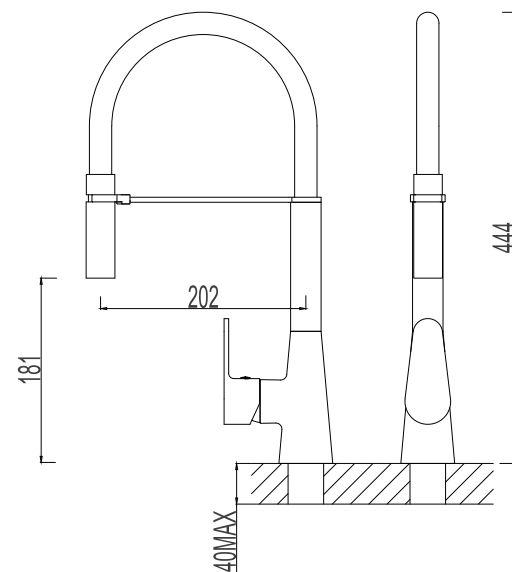
517297-2601 Polished Gold Single lever sink mixer Material: Zinc alloy handle&Brass body With ceramic cartridge&brass aerator With flexible hose&swivel spout Packing:8pcs/ctn
