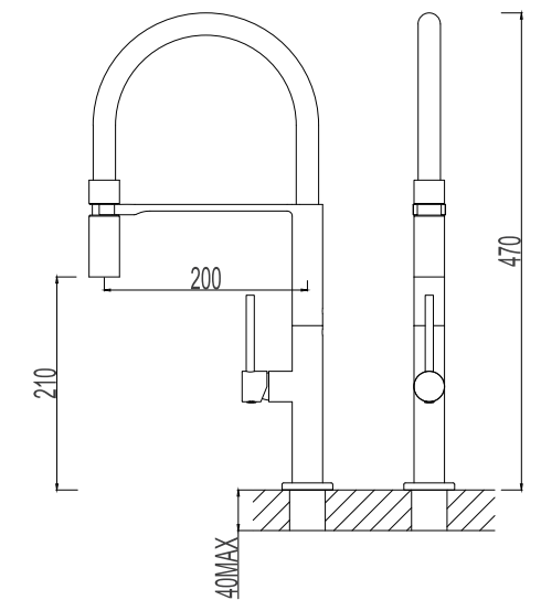
517970-2304 Gun metal black Single lever sink mixer Material: Zinc alloy handle&Brass body With ceramic cartridge&brass aerator With flexible hose&swivel spout Packing:8pcs/ctn
