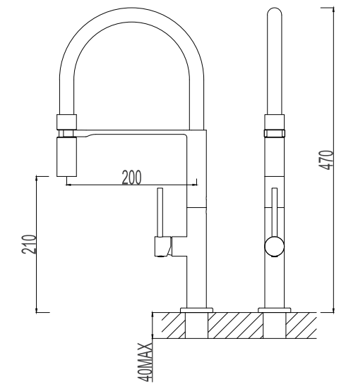
517970-5004 Black Single lever sink mixer Material: Zinc alloy handle&Brass body With ceramic cartridge&brass aerator With flexible hose&swivel spout Packing:8pcs/ctn
