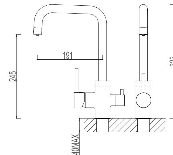
519282-5002 Boiling water tap / Filtered water tap Material: Zinc alloy handle&Brass body With ceramic cartridge&brass aerator With flexible hose&swivel spout Packing:8pcs/ctn
