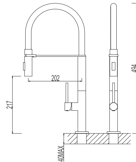
517970-2603 Polished Gold Single lever sink mixer Material: Zinc alloy handle&Brass body With ceramic cartridge&brass aerator With flexible hose&swivel spout Packing:8pcs/ctn
