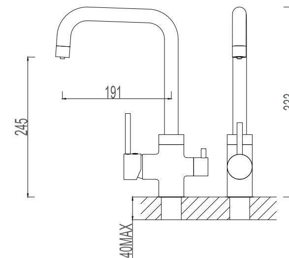
519282-2302 Boiling water tap / Filtered water tap Material: Zinc alloy handle&Brass body With ceramic cartridge&brass aerator With flexible hose&swivel spout Packing:8pcs/ctn
