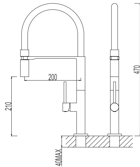
517970-0104 Chrome Single lever sink mixer Material: Zinc alloy handle&Brass body With ceramic cartridge&brass aerator With flexible hose&swivel spout Packing:8pcs/ctn
