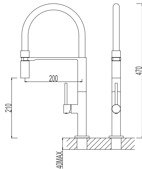
517970-2604 Polished Gold Single lever sink mixer Material: Zinc alloy handle&Brass body With ceramic cartridge&brass aerator With flexible hose&swivel spout Packing:8pcs/ctn
