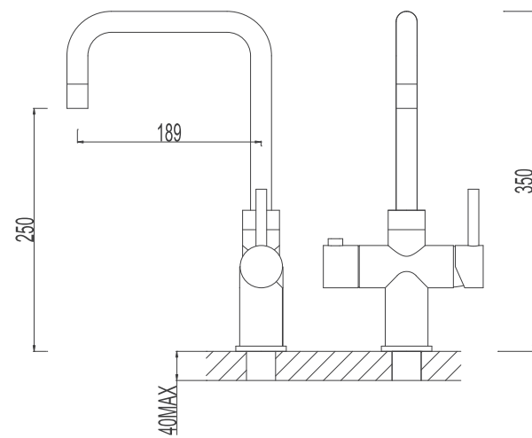
516282-0101 Boiling water tap Material: Zinc alloy handle&Brass body With ceramic cartridge&brass aerator With flexible hose&swivel spout Packing:8pcs/ctn
