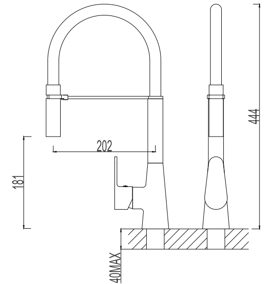
517297-5001 Black Single lever sink mixer Material: Zinc alloy handle&Brass body With ceramic cartridge&brass aerator With flexible hose&swivel spout Packing:8pcs/ctn
