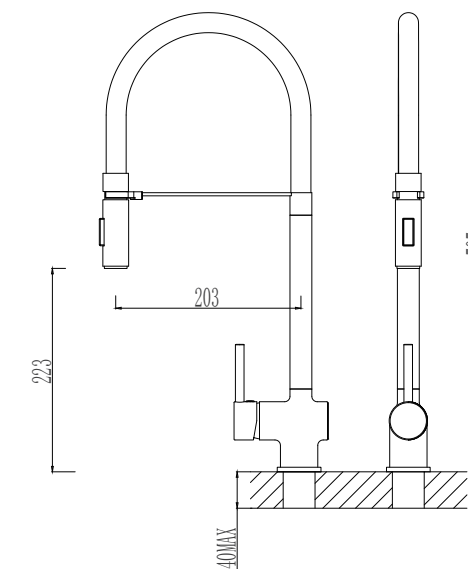
517276-2303 Gun metal black Single lever sink mixer Material: Zinc alloy handle&Brass body With ceramic cartridge&brass aerator With flexible hose&swivel spout Packing:8pcs/ctn
