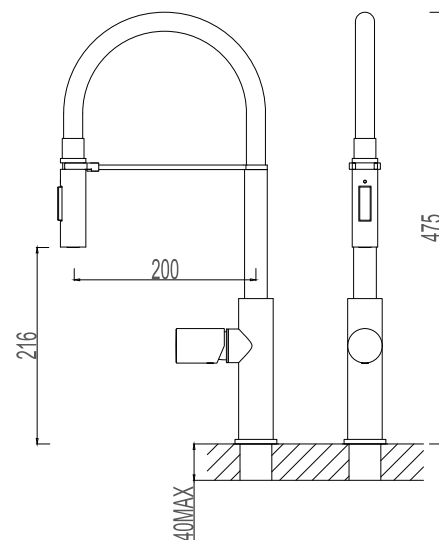
517219-2603 Polished Gold Single lever sink mixer Material: Zinc alloy handle&Brass body With ceramic cartridge&brass aerator With flexible hose&swivel spout Packing:8pcs/ctn
