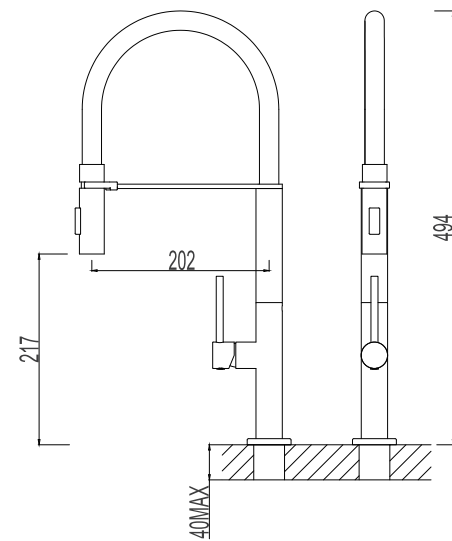
517970-3603 Ø25 Single lever sink mixer Material: Zinc alloy handle&Brass body With ceramic cartridge&brass aerator With flexible hose&swivel spout Packing:8pcs/ctn
