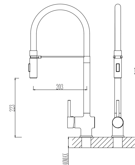
517276-5003 Black Single lever sink mixer Material: Zinc alloy handle&Brass body With ceramic cartridge&brass aerator With flexible hose&swivel spout Packing:8pcs/ctn
