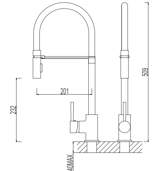
517282-5003 Black Single lever sink mixer Material: Zinc alloy handle&Brass body With ceramic cartridge&brass aerator With flexible hose&swivel spout Packing:8pcs/ctn
