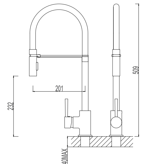
517282-3603 Single lever sink mixer Material: Zinc alloy handle&Brass body With ceramic cartridge&brass aerator With flexible hose&swivel spout Packing:8pcs/ctn
