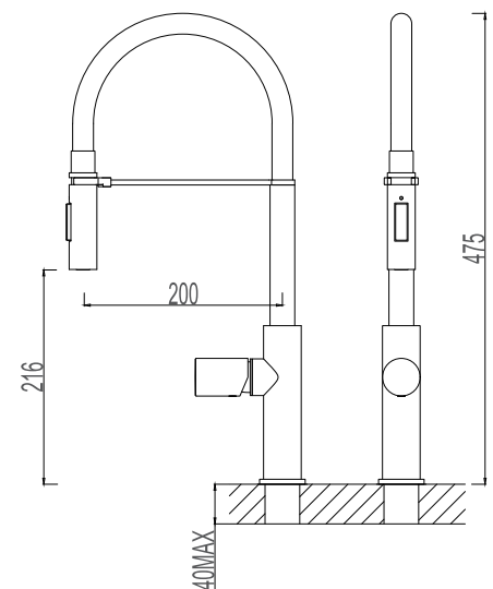
517219-3603 Ø25 Single lever sink mixer Material: Zinc alloy handle&Brass body With ceramic cartridge&brass aerator With flexible hose&swivel spout Packing:8pcs/ctn
