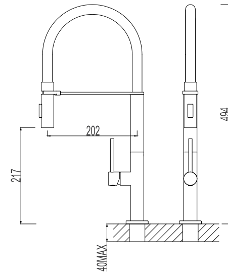
517970-0103 Chrome Single lever sink mixer Material: Zinc alloy handle&Brass body With ceramic cartridge&brass aerator With flexible hose&swivel spout Packing:8pcs/ctn
