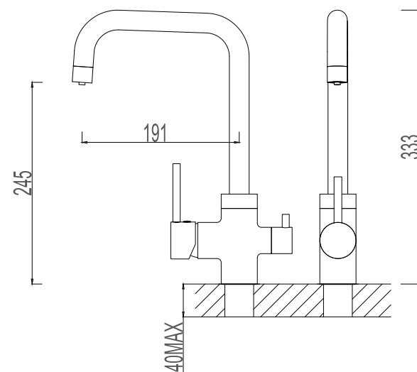
519282-1102 Boiling water tap / Filtered water tap Material: Zinc alloy handle&Brass body With ceramic cartridge&brass aerator With flexible hose&swivel spout Packing:8pcs/ctn
