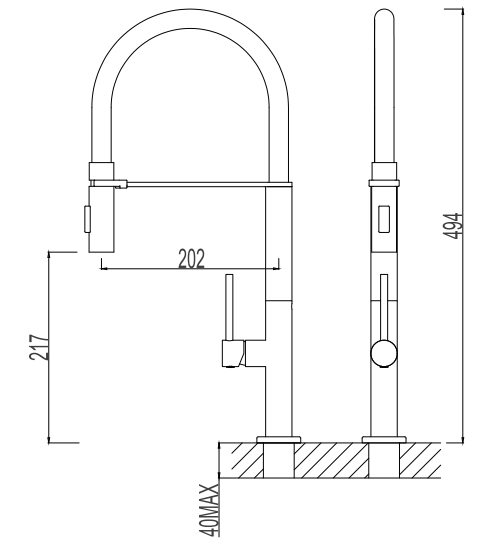
517970-5003 Black Single lever sink mixer Material: Zinc alloy handle&Brass body With ceramic cartridge&brass aerator With flexible hose&swivel spout Packing:8pcs/ctn
