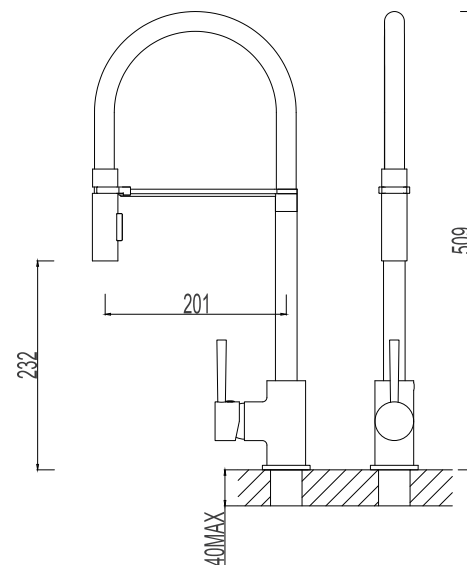
517282-2603 Polished Gold Single lever sink mixer Material: Zinc alloy handle&Brass body With ceramic cartridge&brass aerator With flexible hose&swivel spout Packing:8pcs/ctn
