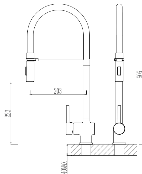
517276-2603 Polished Gold Single lever sink mixer Material: Zinc alloy handle&Brass body With ceramic cartridge&brass aerator With flexible hose&swivel spout Packing:8pcs/ctn
