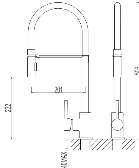
517282-0103 Chrome Single lever sink mixer Material: Zinc alloy handle&Brass body With ceramic cartridge&brass aerator With flexible hose&swivel spout Packing:8pcs/ctn
