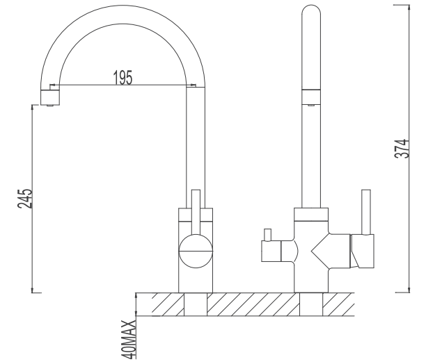
516282-0102 Boiling water tap Material: Zinc alloy handle&Brass body With ceramic cartridge&brass aerator With flexible hose&swivel spout Packing:8pcs/ctn
