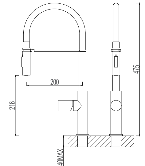
517219-5003 Black Single lever sink mixer Material: Zinc alloy handle&Brass body With ceramic cartridge&brass aerator With flexible hose&swivel spout Packing:8pcs/ctn
