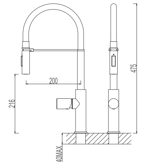
517219-2303 Gun metal black Single lever sink mixer Material: Zinc alloy handle&Brass body With ceramic cartridge&brass aerator With flexible hose&swivel spout Packing:8pcs/ctn
