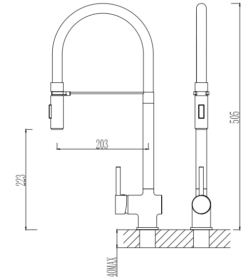
517276-3603 Single lever sink mixer Material: Zinc alloy handle&Brass body With ceramic cartridge&brass aerator With flexible hose&swivel spout Packing:8pcs/ctn
