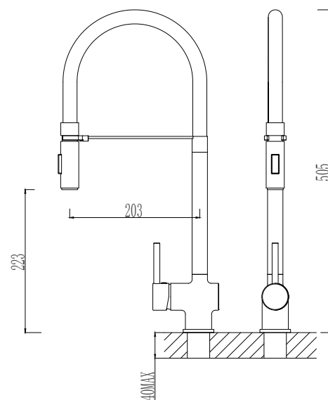
517276-0103 Chrome Single lever sink mixer Material: Zinc alloy handle&Brass body With ceramic cartridge&brass aerator With flexible hose&swivel spout Packing:8pcs/ctn
