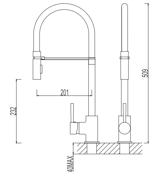
517282-2303 Gun metal black Single lever sink mixer Material: Zinc alloy handle&Brass body With ceramic cartridge&brass aerator With flexible hose&swivel spout Packing:8pcs/ctn
