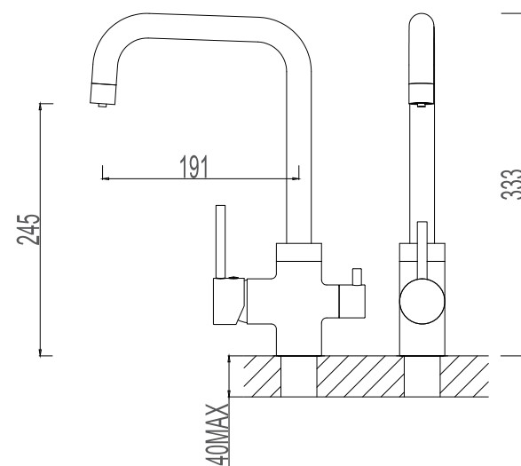
519282-0102 Boiling water tap / Filtered water tap Material: Zinc alloy handle&Brass body With ceramic cartridge&brass aerator With flexible hose&swivel spout Packing:8pcs/ctn
