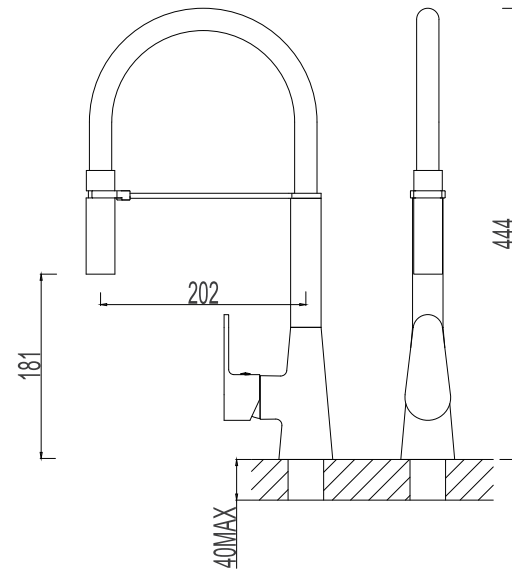
517297-0101 Chrome Single lever sink mixer Material: Zinc alloy handle&Brass body With ceramic cartridge&brass aerator With flexible hose&swivel spout Packing:8pcs/ctn
