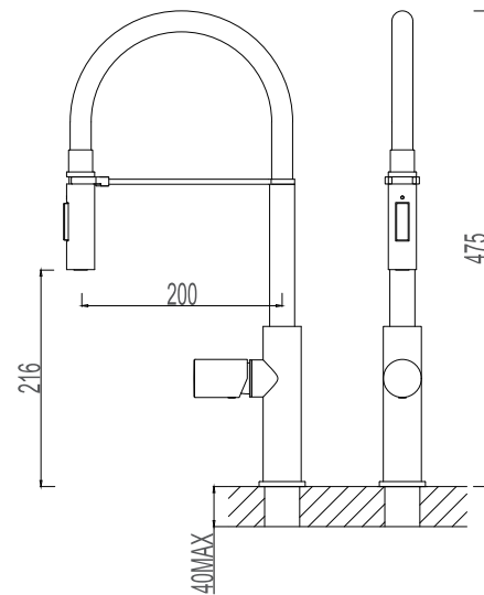
517219-0103 Chrome Single lever sink mixer Material: Zinc alloy handle&Brass body With ceramic cartridge&brass aerator With flexible hose&swivel spout Packing:8pcs/ctn
