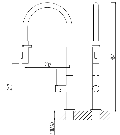
517970-2303 Gun metal black Single lever sink mixer Material: Zinc alloy handle&Brass body With ceramic cartridge&brass aerator With flexible hose&swivel spout Packing:8pcs/ctn
