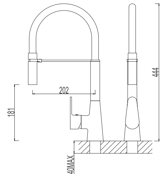
517297-2301 Gun metal black Single lever sink mixer Material: Zinc alloy handle&Brass body With ceramic cartridge&brass aerator With flexible hose&swivel spout Packing:8pcs/ctn
